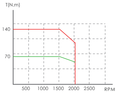
MVM7-M20D-01115-□1FNS
