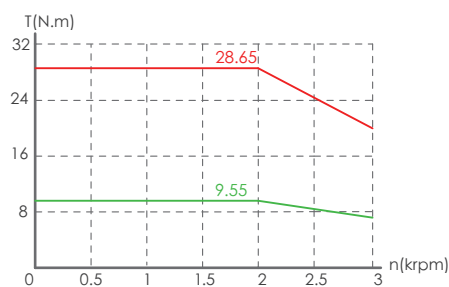
MV7E-M13□-2R020-□□
