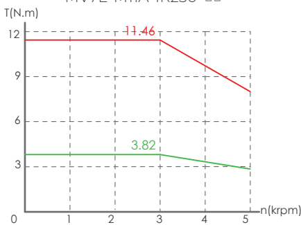
MV7E-M11A-1R230-□□
