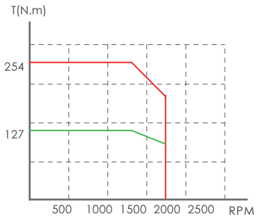
MVM7-M20D-02015-□1FN
