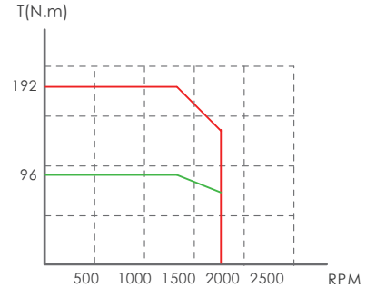
MVM7-M20D-01515-□1FNS
