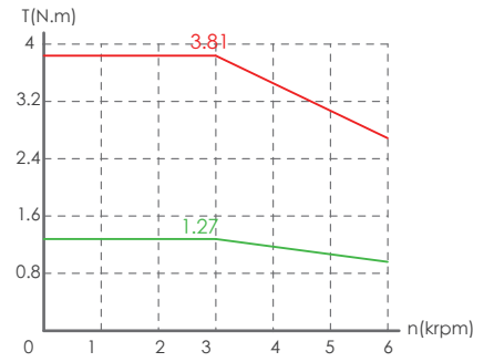
MV7E-□06A-R4030-□□
