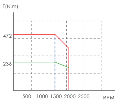
MV7-M26D-03715-□1FN
