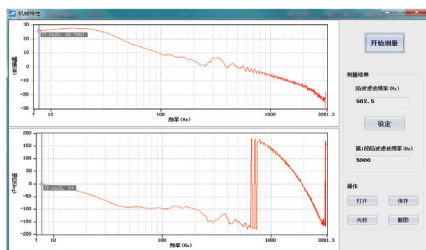
Mechanical characteristics analysis, automatic resonance suppression
