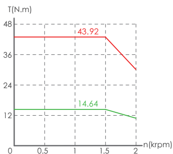
MV7E-M13□-2R315-□□L
