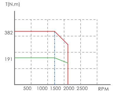
MVM7-M26D-03015-□1FN
