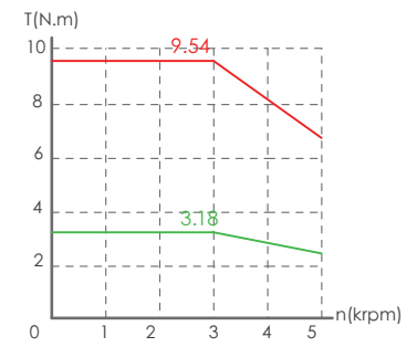
MV7E-L08A-1R030-□□
