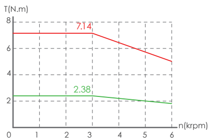
MV7E-M11A-1R230-□□
