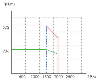
MV7-M26D-04515-□1FN
