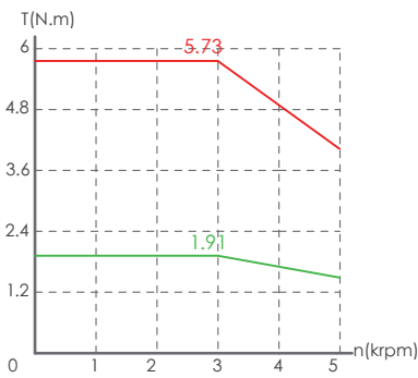
MV7E-□08A-R7530-□□
