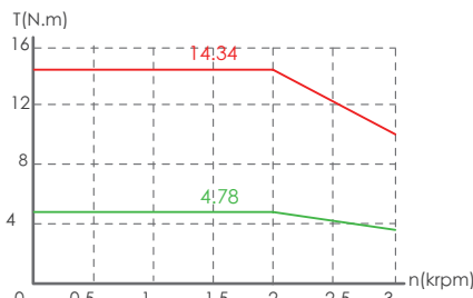
MV7E-M13-□1R020-□□
