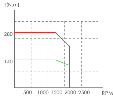
MVM7-M20D-02215-□1FN
