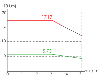
MV7E-M11A-1R830-□□
