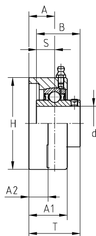
SUCFL200
