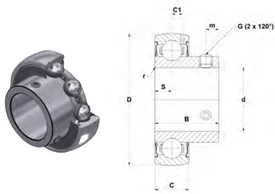
US..G2
