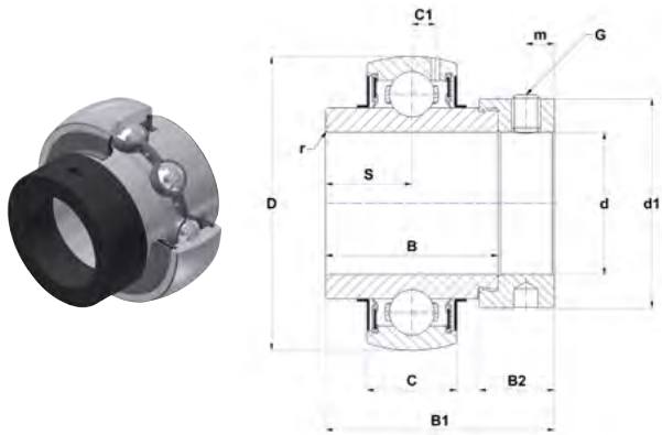
EX..G2T04
