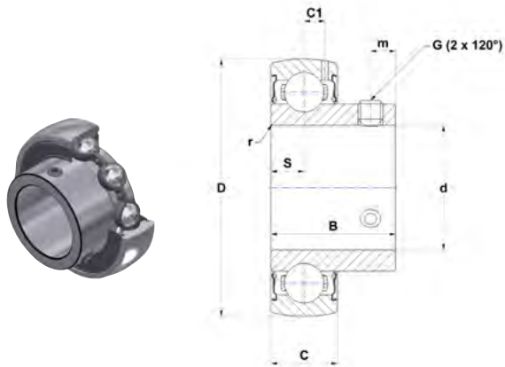
US..G2
