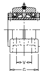
FOUR BOLT
