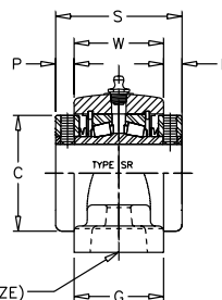
TWO BOLT
