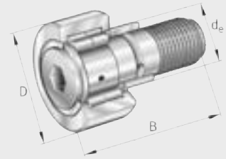
PWKRE...-2RS
